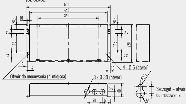
Interfejs LonWorks (CZ-CLNC2)
